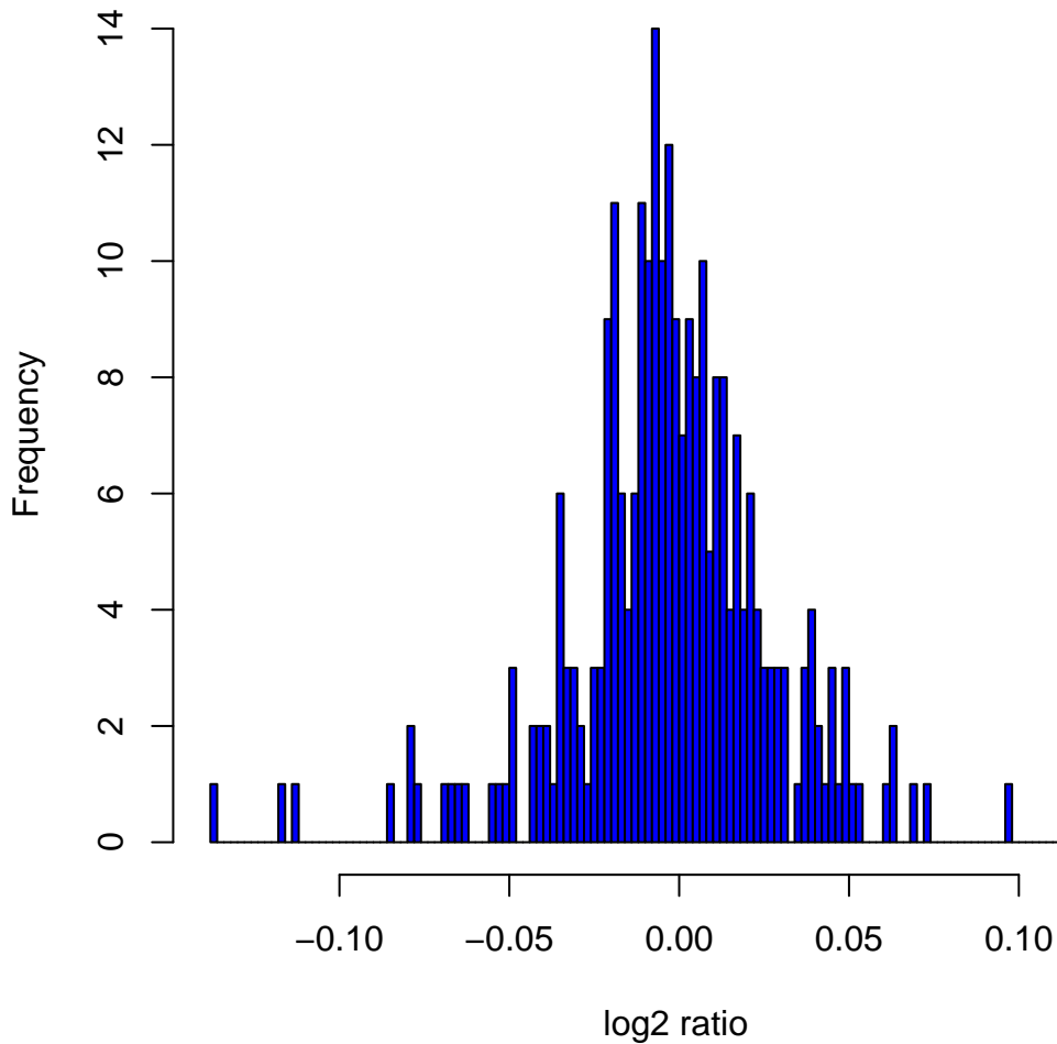
Histogram of \log_2 ratios in 270 HapMap samples at clone Chr9tp-9D3
