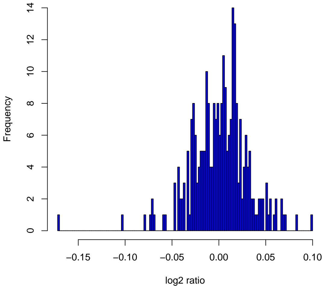
Histogram of log 2 ratios in 270 HapMap samples at clone Chr9tp-9E1
