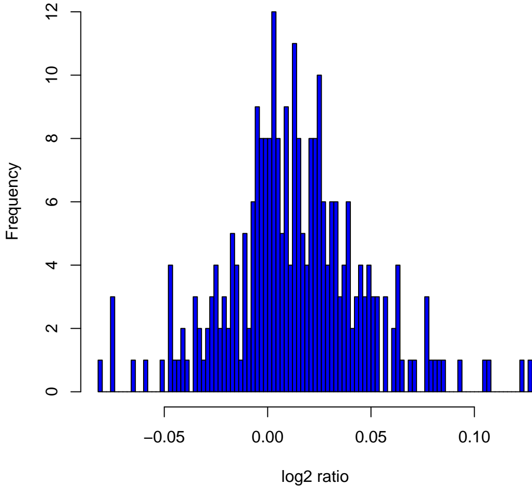
Histogram of log2ratios in 270 HapMap samples at clone Chr9tp-9G12
