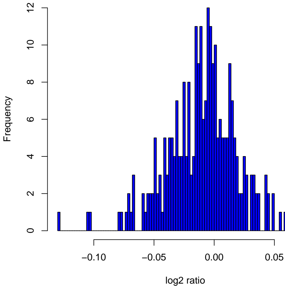
Histogram of \log_2 ratios in 270 HapMap samples at clone Chr9tp-9H4
