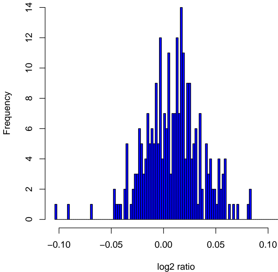
Histogram of log2ratios in 270 HapMap samples at clone Chr9tp-9H9
