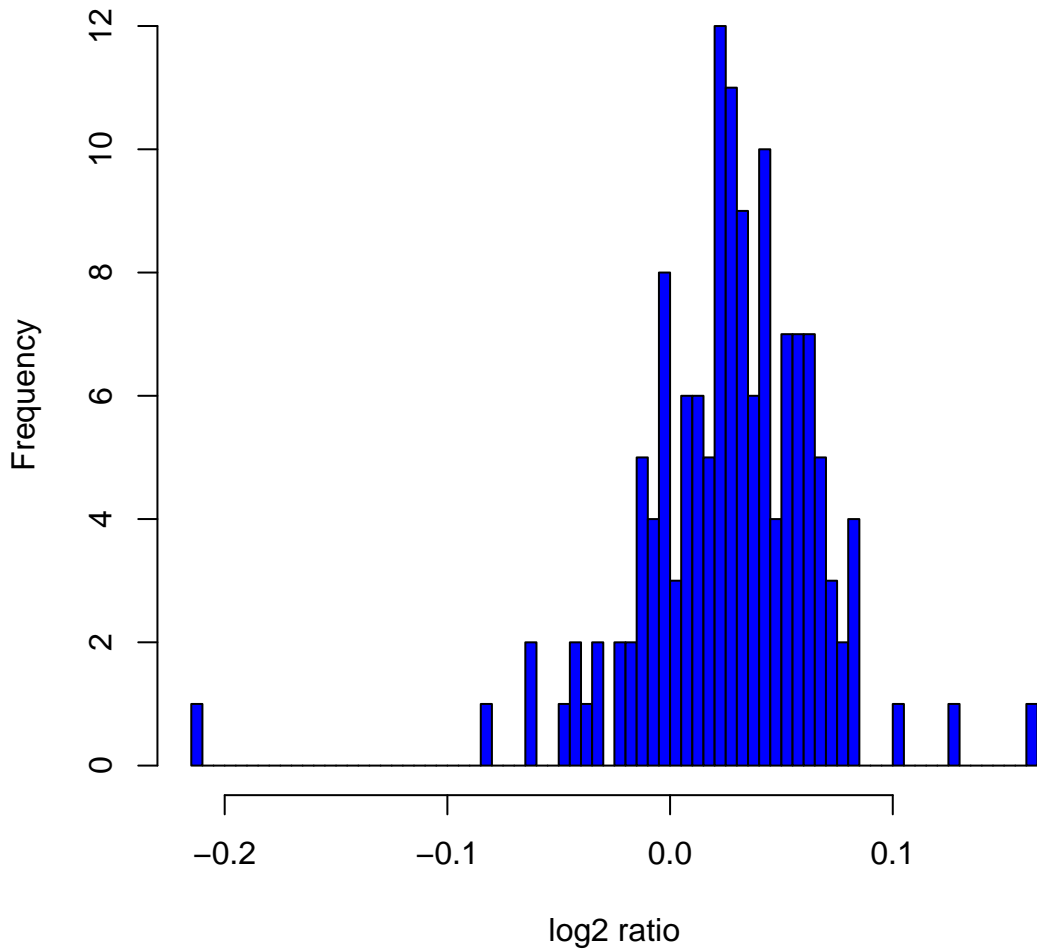
Histogram of log 2 ratios in 142 HapMap male samples at clone ChrXtp-10C1
