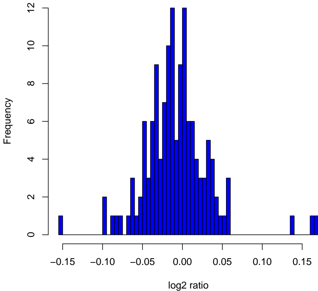
Histogram of \log_2 ratios in 142 HapMap male samples at clone ChrXtp-10C5
