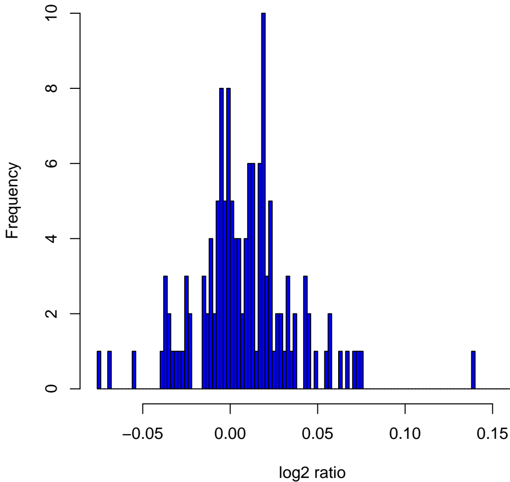
Histogram of \log_2 ratios in 142 HapMap male samples at clone ChrXtp-10C8
