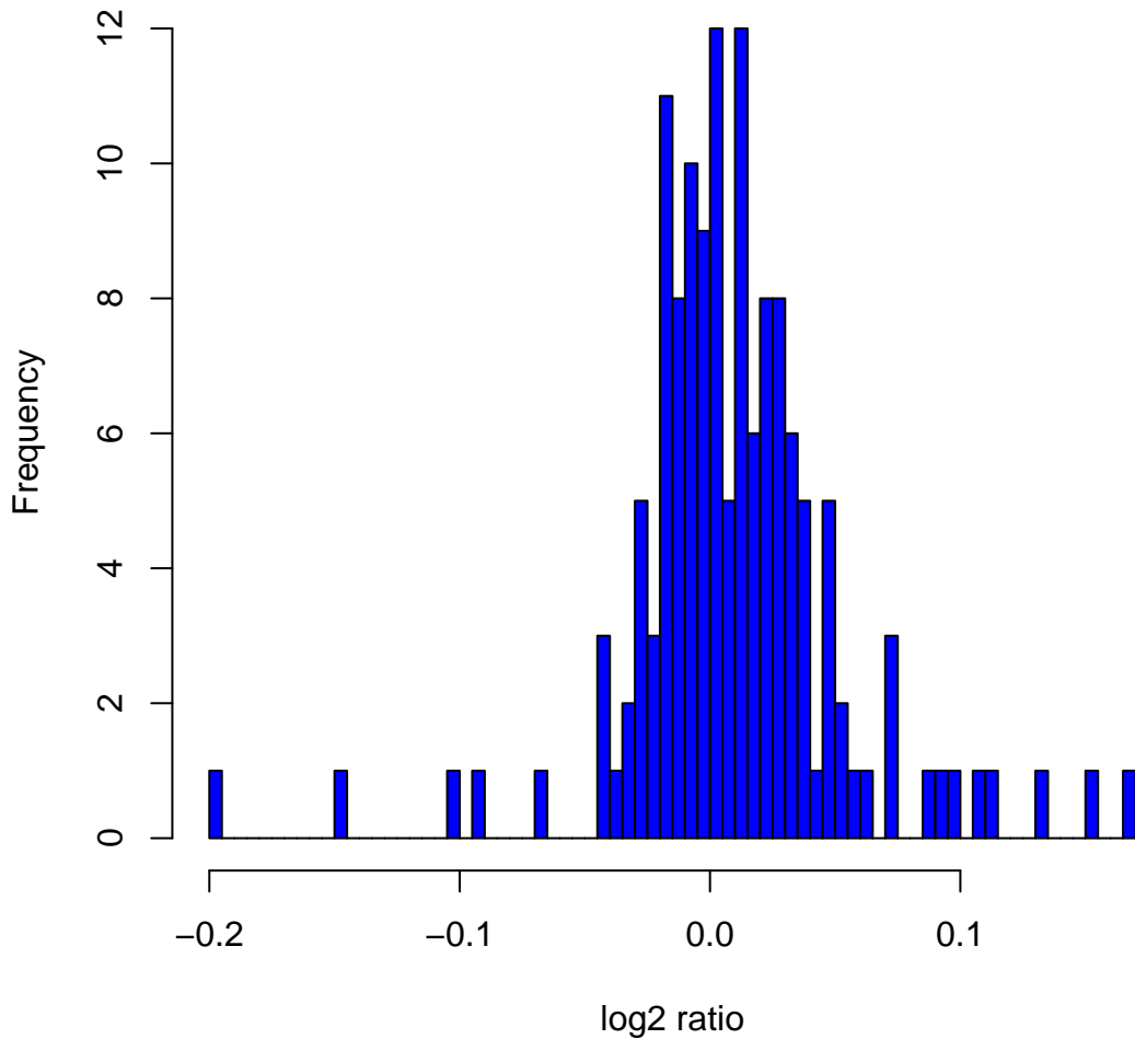
Histogram of log2ratios in 142 HapMap male samples at clone ChrXtp-10C9
