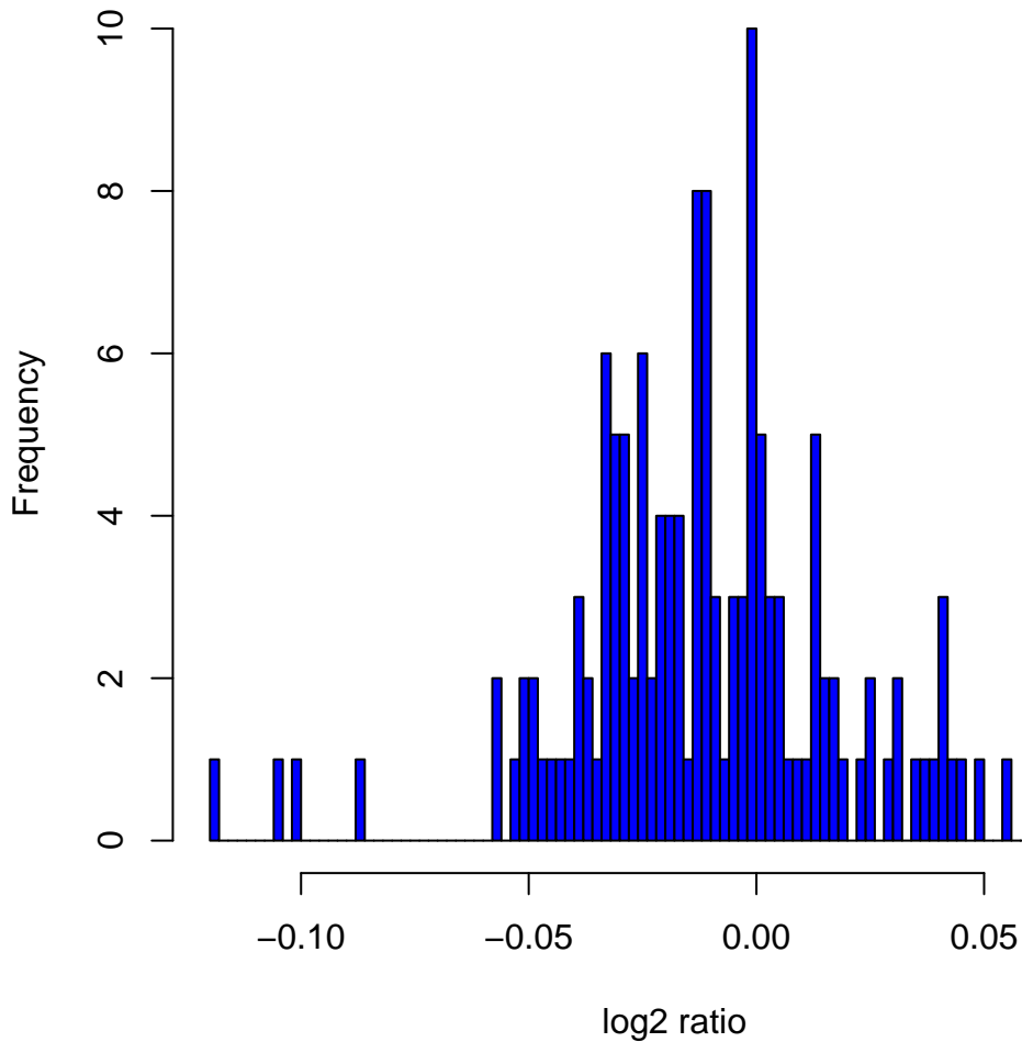
Histogram of log 2 ratios in 142 HapMap male samples at clone ChrXtp-10G11
