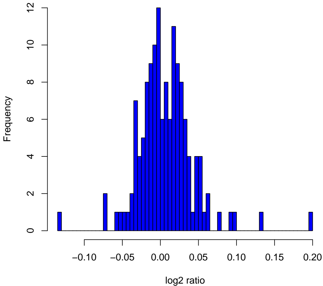
Histogram of \log_2 ratios in 142 HapMap male samples at clone ChrXtp-10H9
