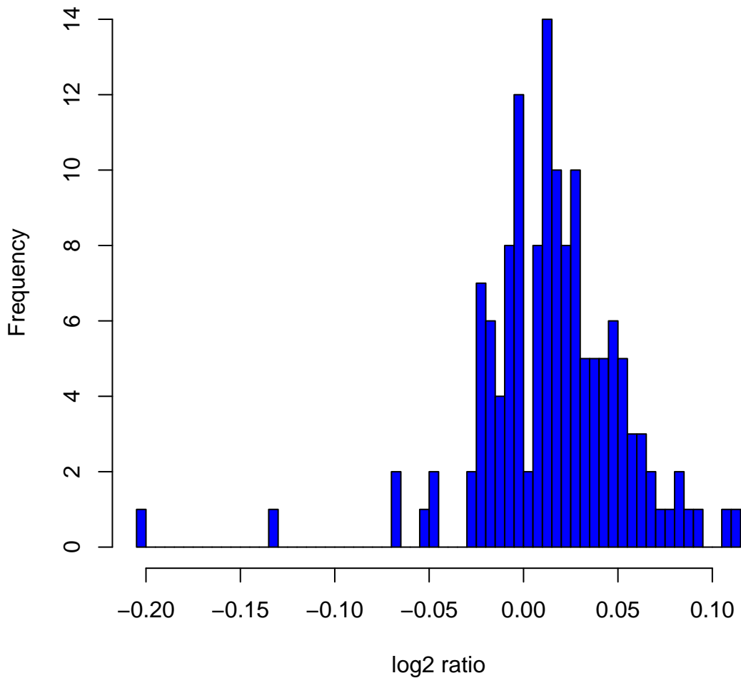
Histogram of log 2 ratios in 142 HapMap male samples at clone ChrXtp-11A10
