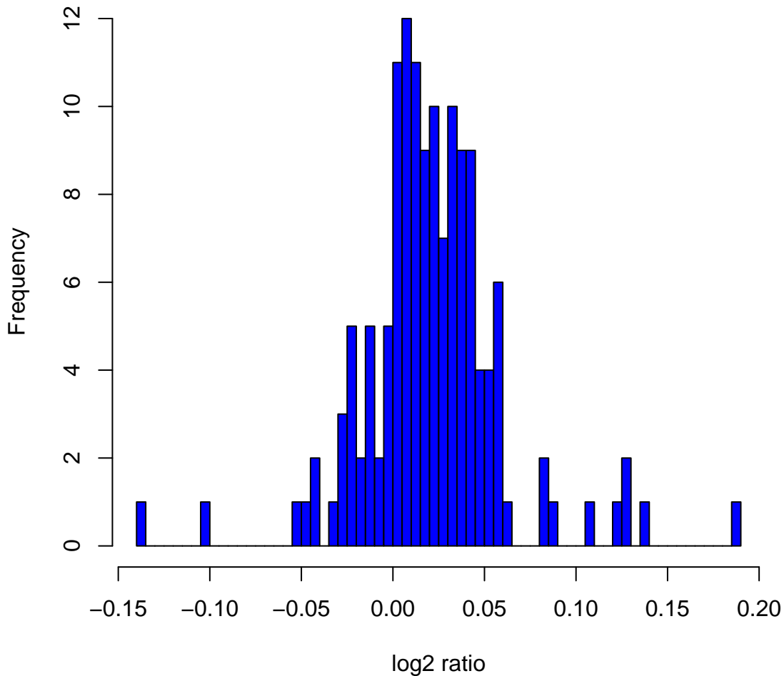
Histogram of log 2 ratios in 142 HapMap male samples at clone ChrXtp-11A2
