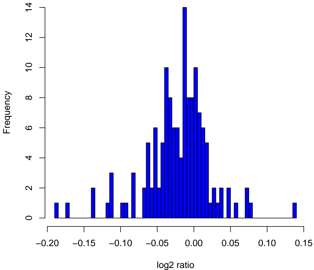
Histogram of log 2 ratios in 142 HapMap male samples at clone ChrXtp-11C3
