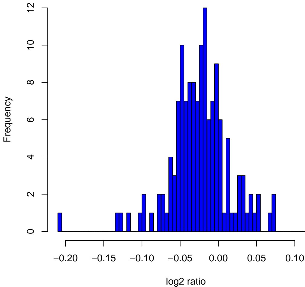
Histogram of log 2 ratios in 142 HapMap male samples at clone ChrXtp-11F2
