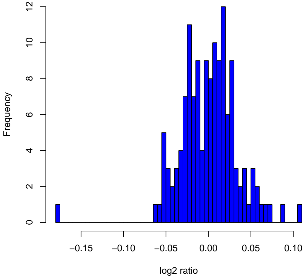
Histogram of log2ratios in 142 HapMap male samples at clone ChrXtp-11F7
