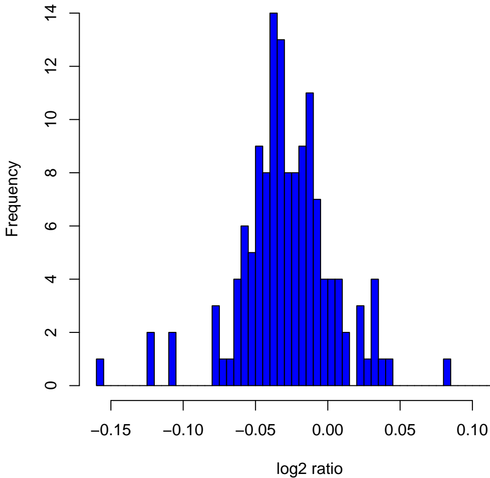
Histogram of log 2 ratios in 142 HapMap male samples at clone ChrXtp-11G2
