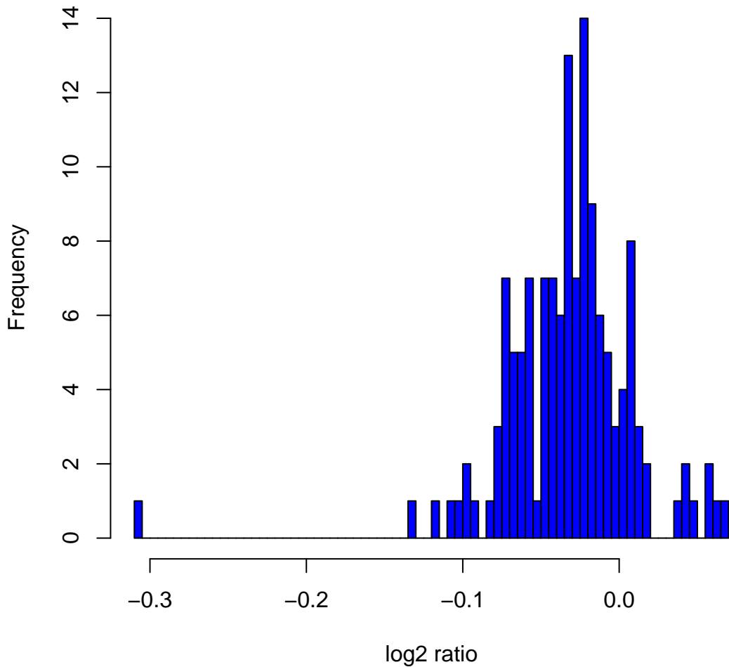
Histogram of log 2 ratios in 142 HapMap male samples at clone ChrXtp-11G3
