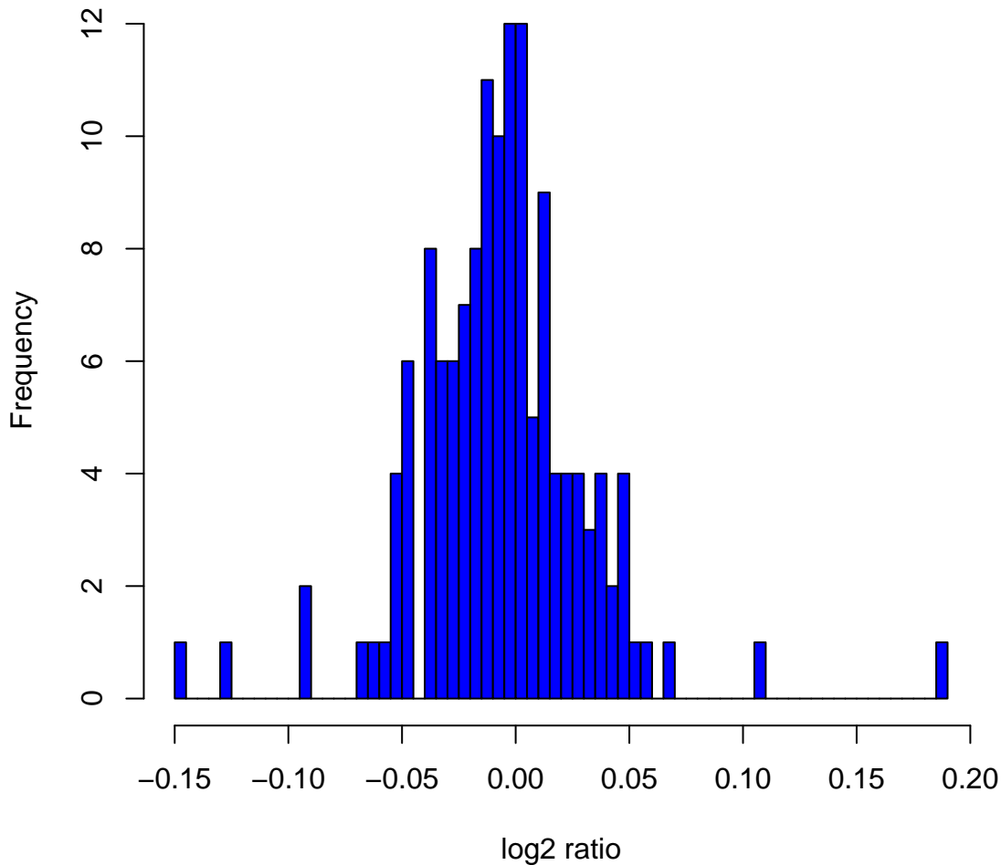
Histogram of \log_2 ratios in 142 HapMap male samples at clone ChrXtp-11G4
