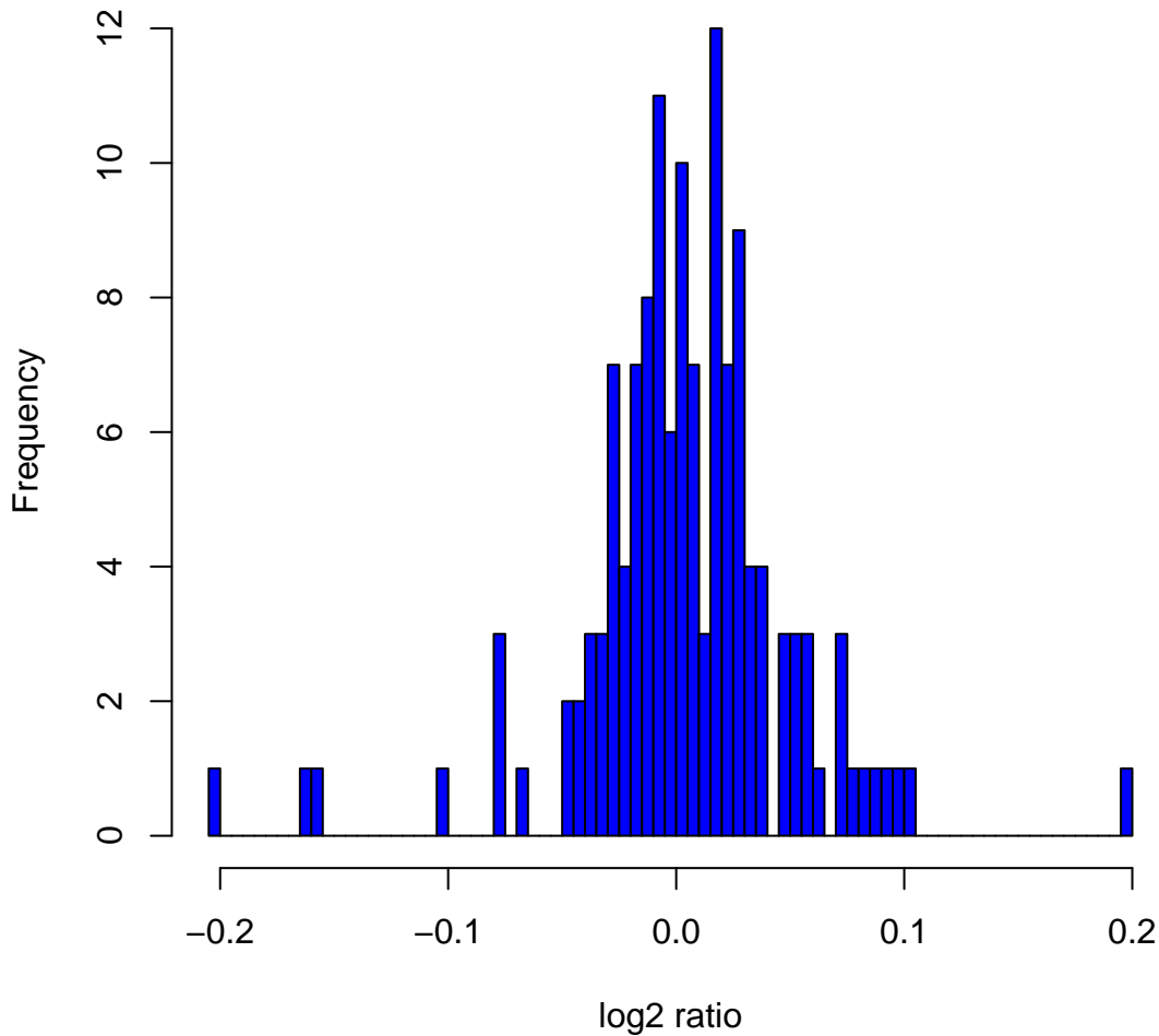
Histogram of log 2 ratios in 142 HapMap male samples at clone ChrXtp-11H1
