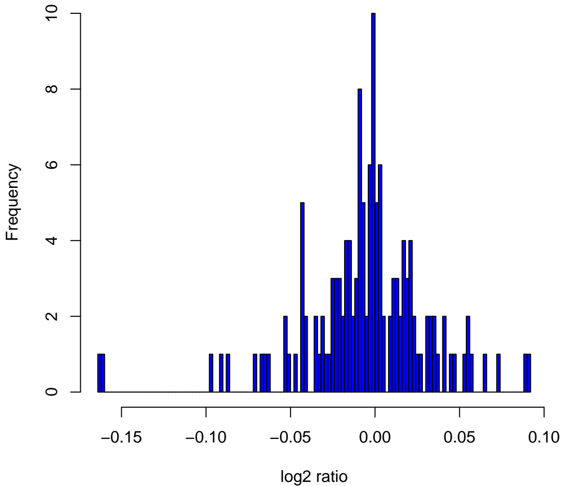
Histogram of log 2 ratios in 142 HapMap male samples at clone ChrXtp-12E8
