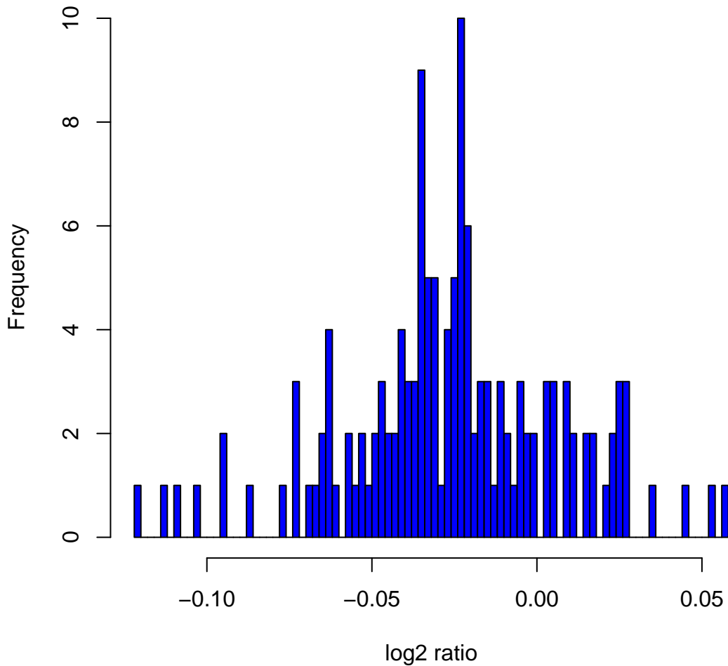
Histogram of log 2 ratios in 142 HapMap male samples at clone ChrXtp-12G12
