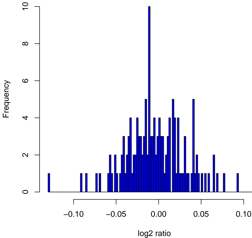
Histogram of log 2 ratios in 142 HapMap male samples at clone ChrXtp-12G7
