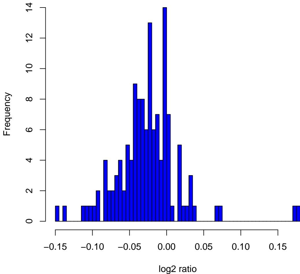
Histogram of log 2 ratios in 142 HapMap male samples at clone ChrXtp-14A12
