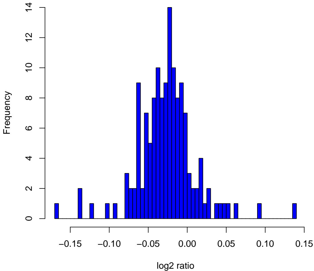
Histogram of \log_2 ratios in 142 HapMap male samples at clone ChrXtp-15A5
