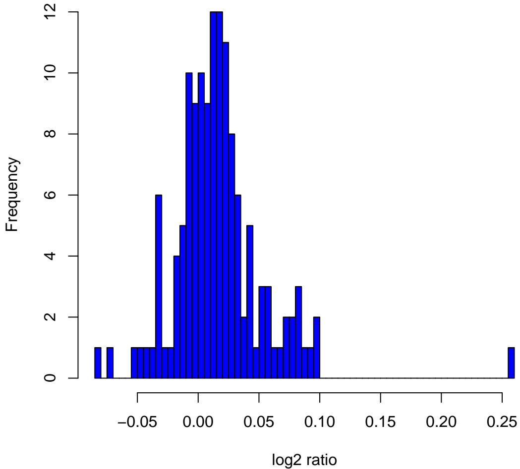
Histogram of \log_2 ratios in 142 HapMap male samples at clone ChrXtp-17B2
