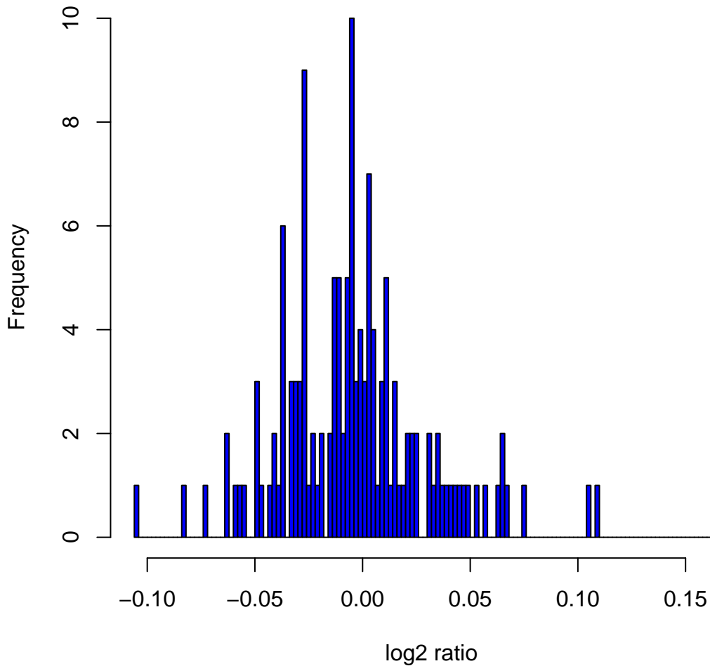
Histogram of \log_2 ratios in 142 HapMap male samples at clone ChrXtp-18A3
