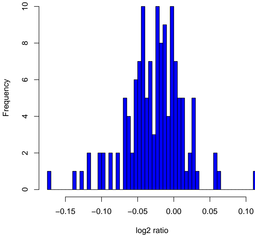
Histogram of log2ratios in 142 HapMap male samples at clone ChrXtp-18D7
