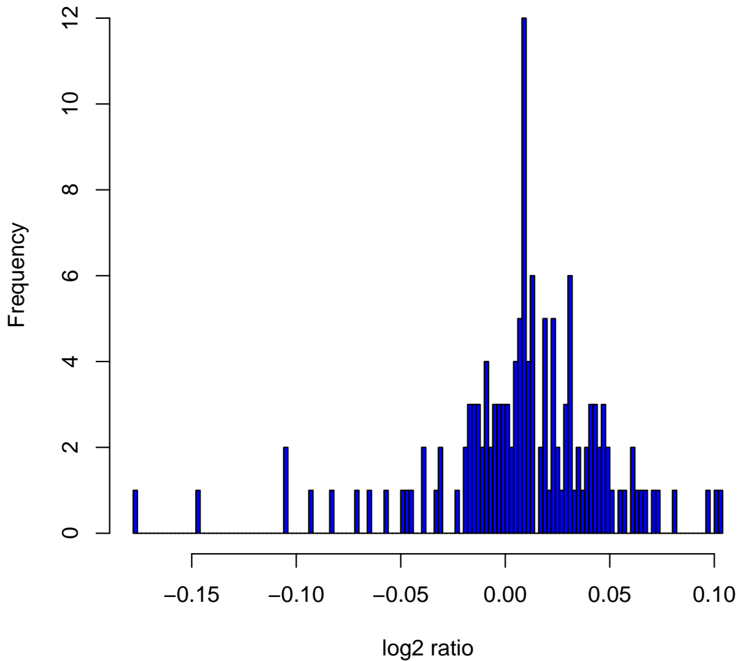
Histogram of log 2 ratios in 142 HapMap male samples at clone ChrXtp-19A2
