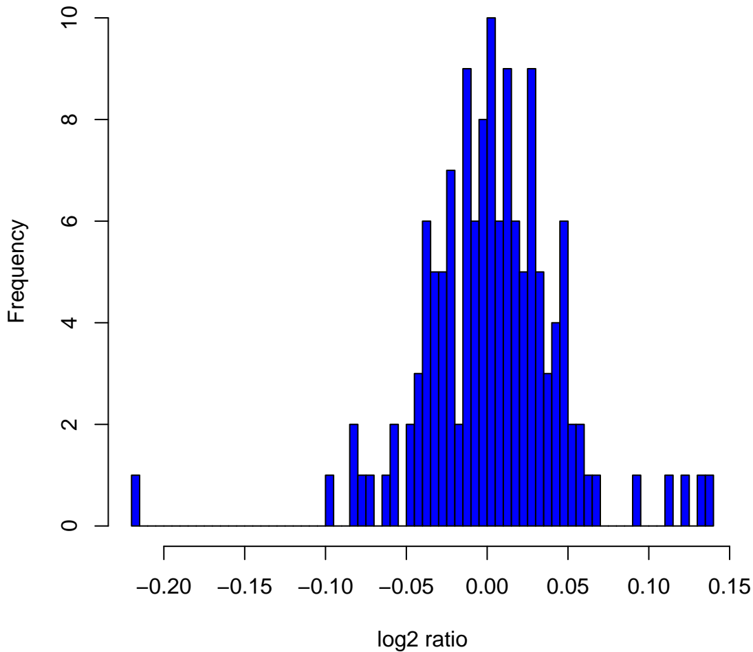
Histogram of log 2 ratios in 142 HapMap male samples at clone ChrXtp-19D3
