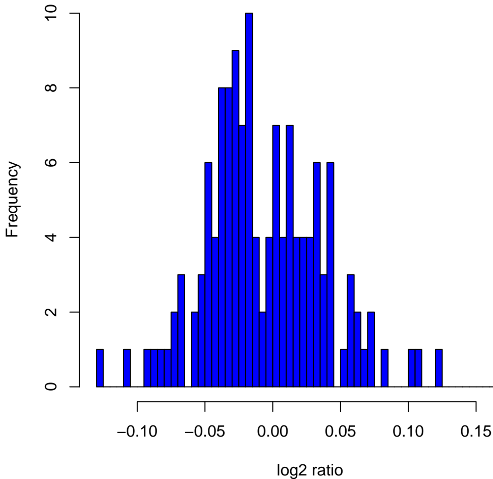
Histogram of \log_2 ratios in 142 HapMap male samples at clone ChrXtp-19F1
