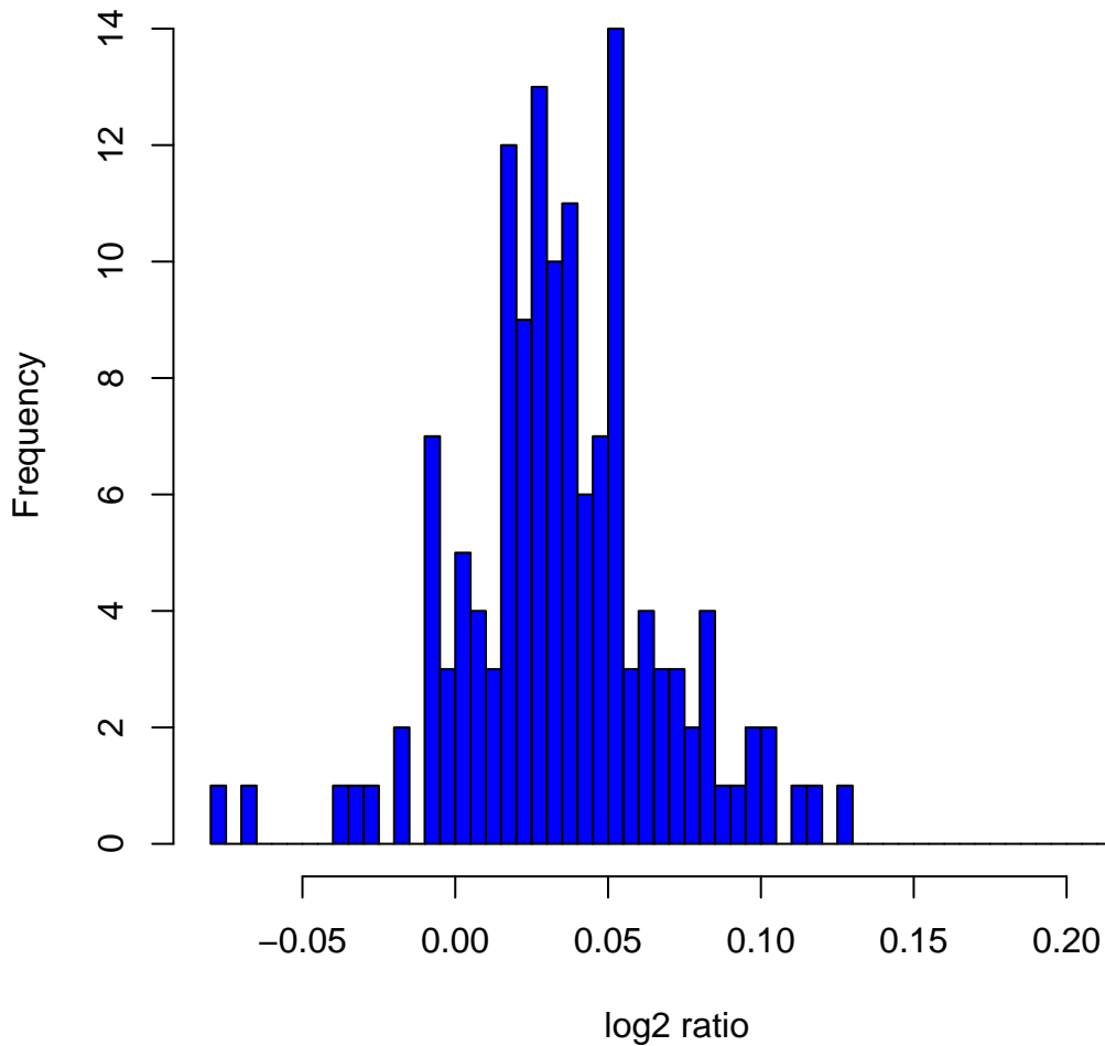
Histogram of log 2 ratios in 142 HapMap male samples at clone ChrXtp-19G11
