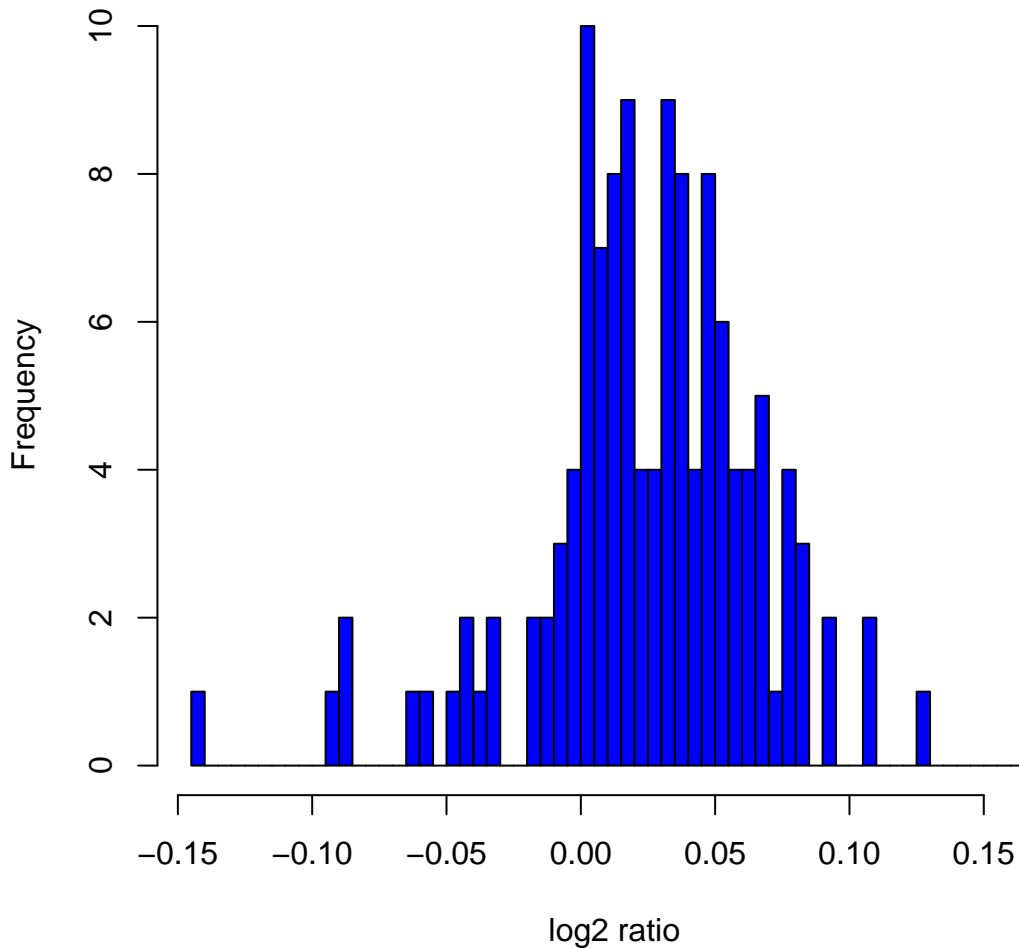
Histogram of log 2 ratios in 142 HapMap male samples at clone ChrXtp-19G5
