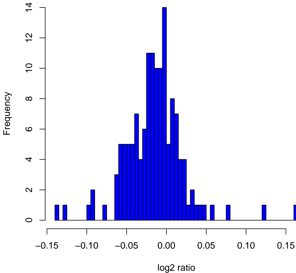
Histogram of log2ratios in 142 HapMap male samples at clone ChrXtp-21A7
