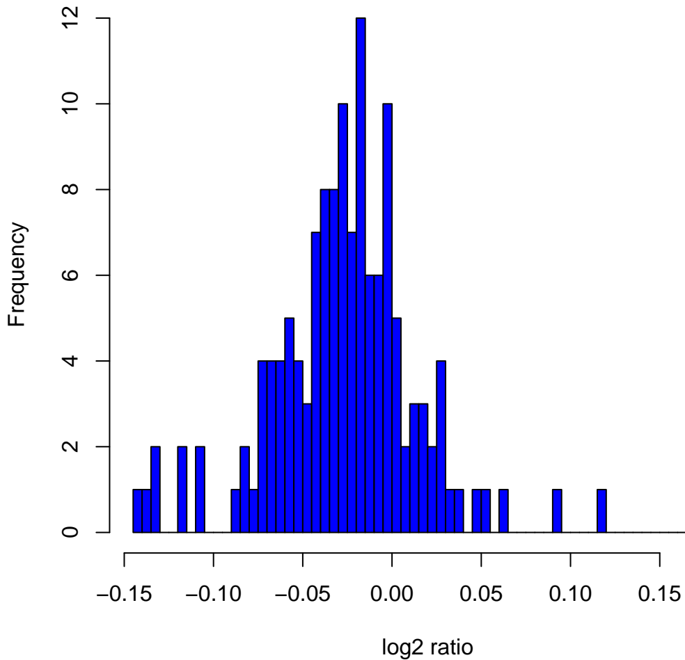
Histogram of log 2 ratios in 142 HapMap male samples at clone ChrXtp-21B3
