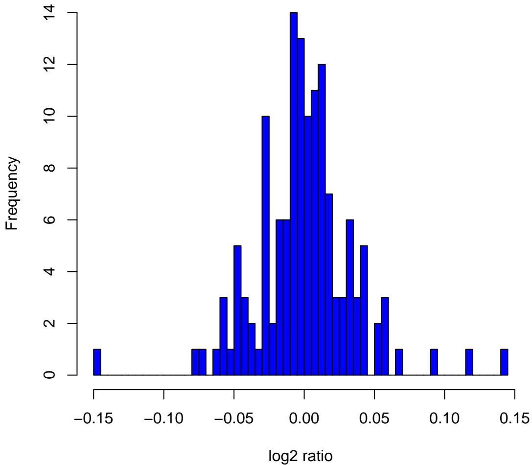
Histogram of log2ratios in 142 HapMap male samples at clone ChrXtp-21D5
