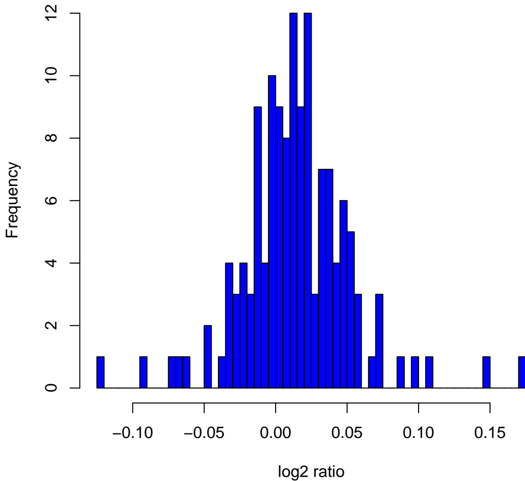
Histogram of \log_2 ratios in 142 HapMap male samples at clone ChrXtp-21F3
