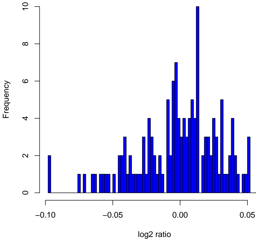
Histogram of log 2 ratios in 142 HapMap male samples at clone ChrXtp-21F6
