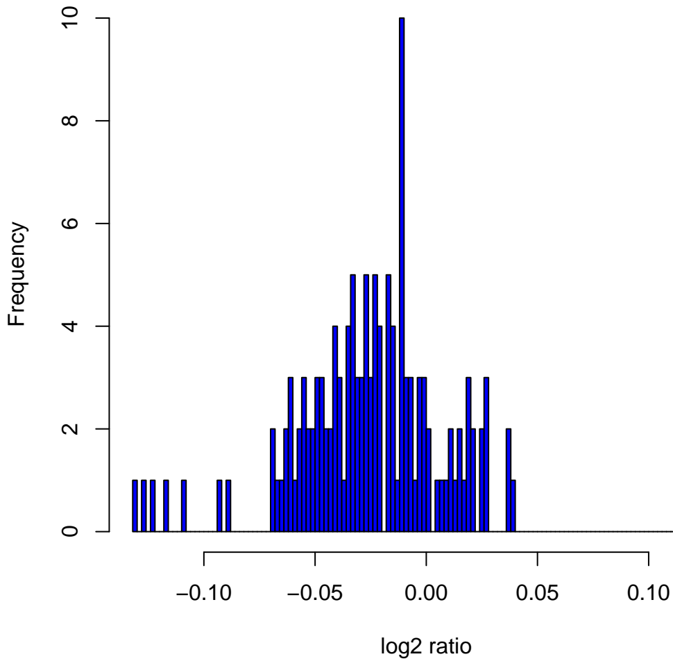
Histogram of log 2 ratios in 142 HapMap male samples at clone ChrXtp-21G5
