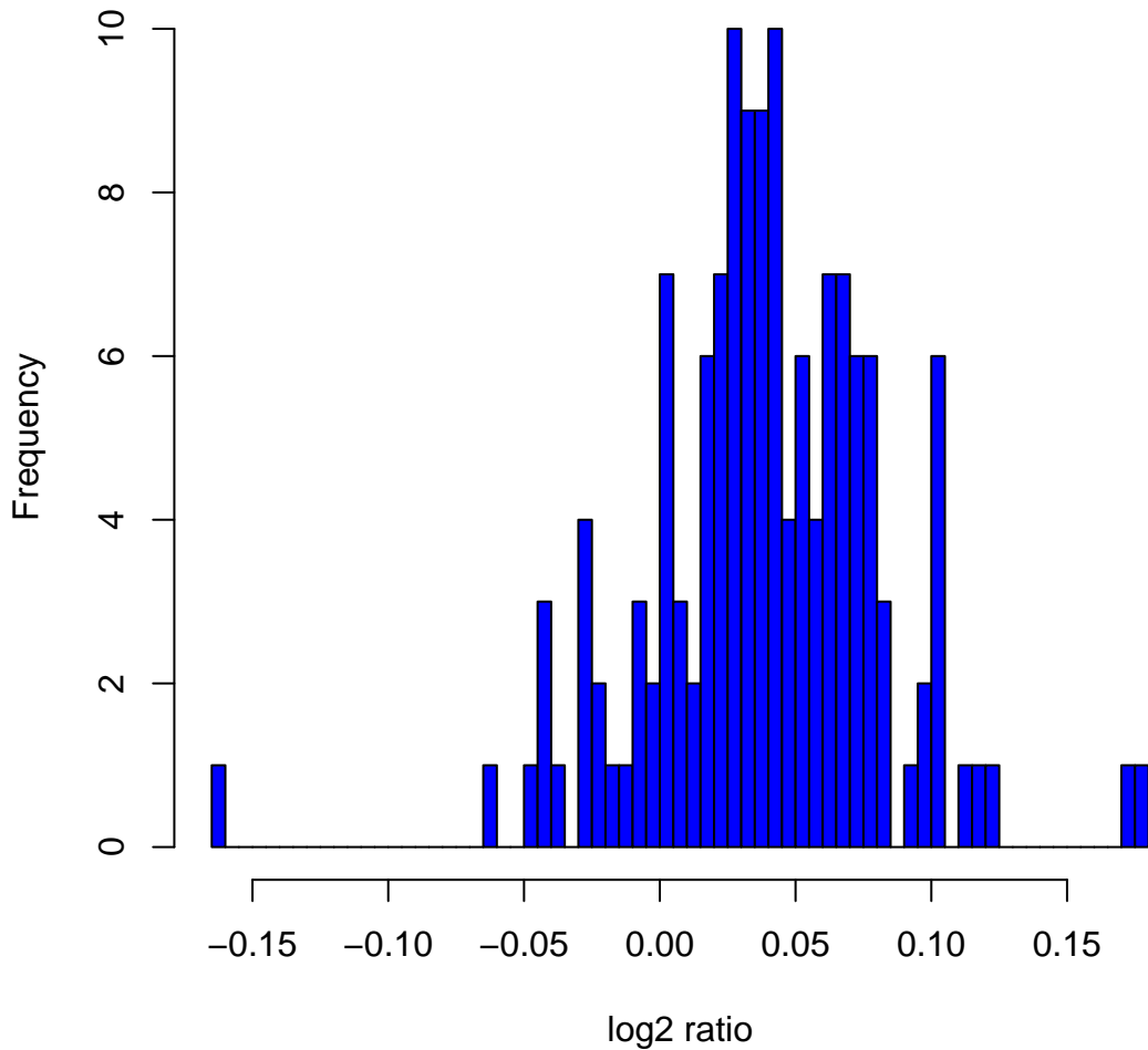
Histogram of log 2 ratios in 142 HapMap male samples at clone ChrXtp-21G7
