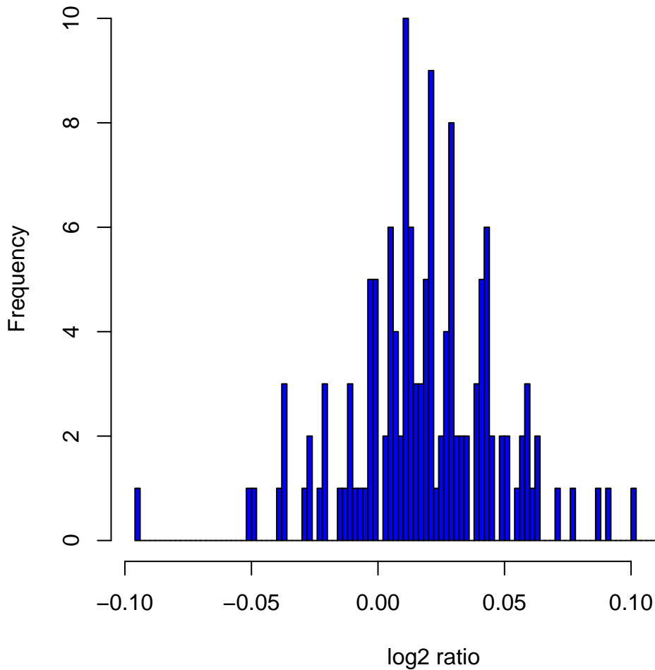
Histogram of log 2 ratios in 142 HapMap male samples at clone ChrXtp-22B7
