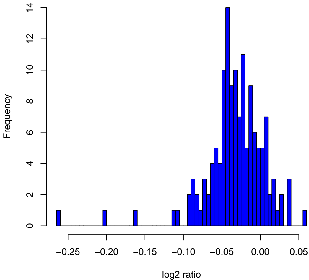
Histogram of log 2 ratios in 142 HapMap male samples at clone ChrXtp-22F2
