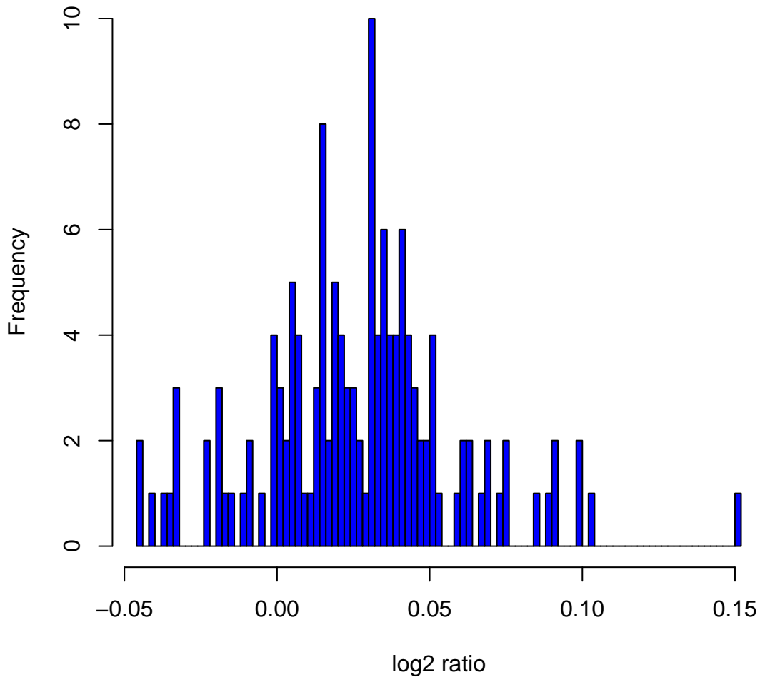
Histogram of \log_2 ratios in 142 HapMap male samples at clone ChrXtp-22G3
