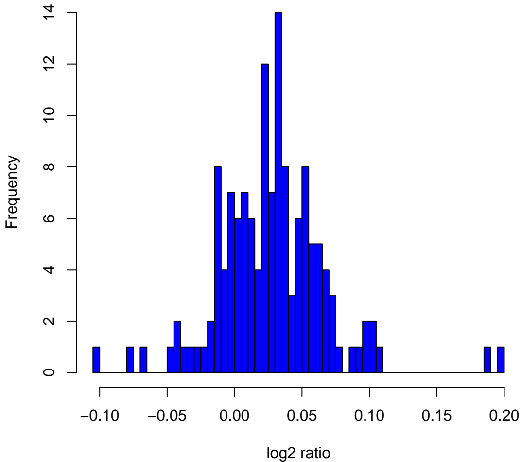
Histogram of \log_2 ratios in 142 HapMap male samples at clone ChrXtp-23A4
