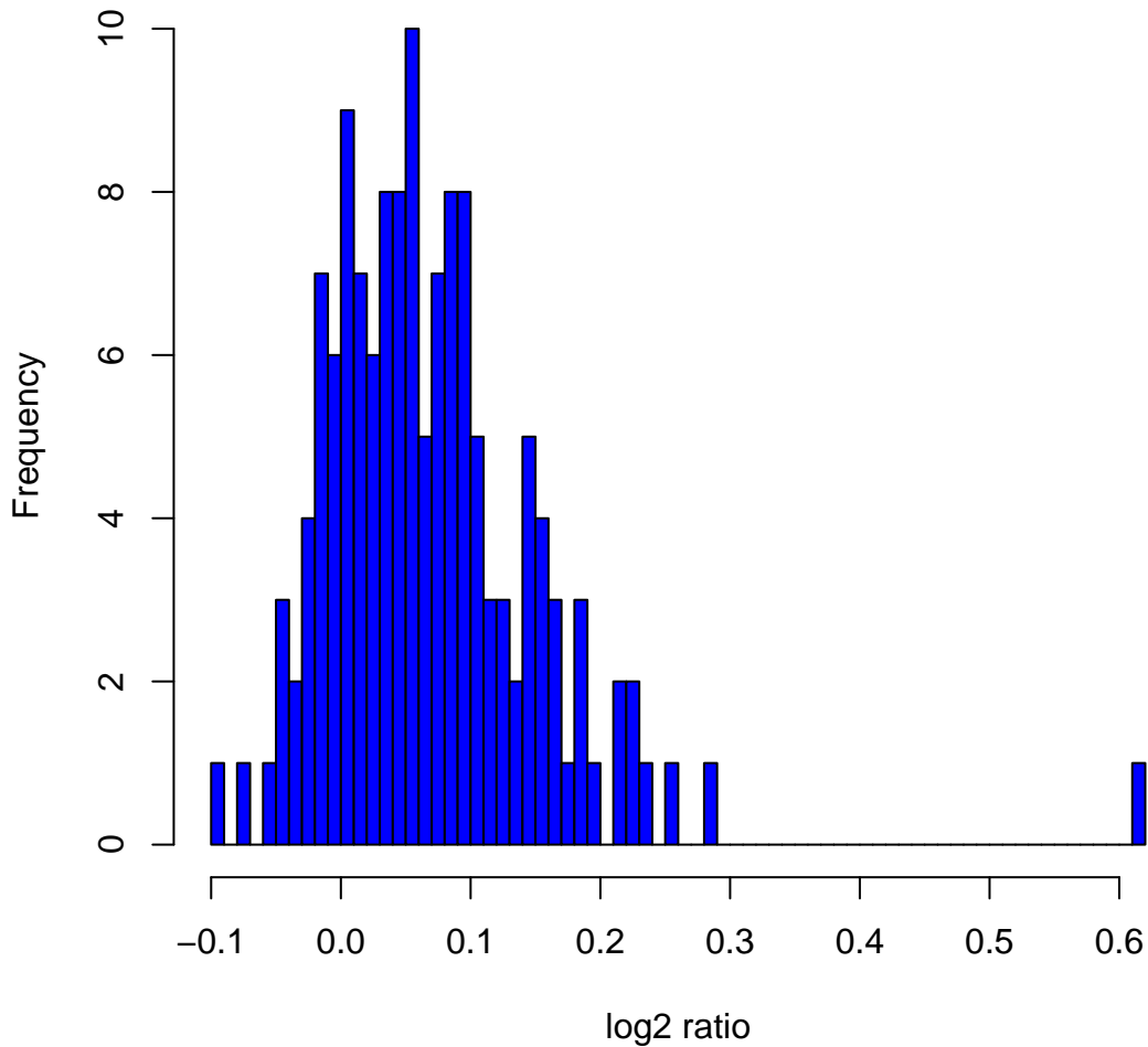
Histogram of \log_2 ratios in 142 HapMap male samples at clone ChrXtp-23A6
