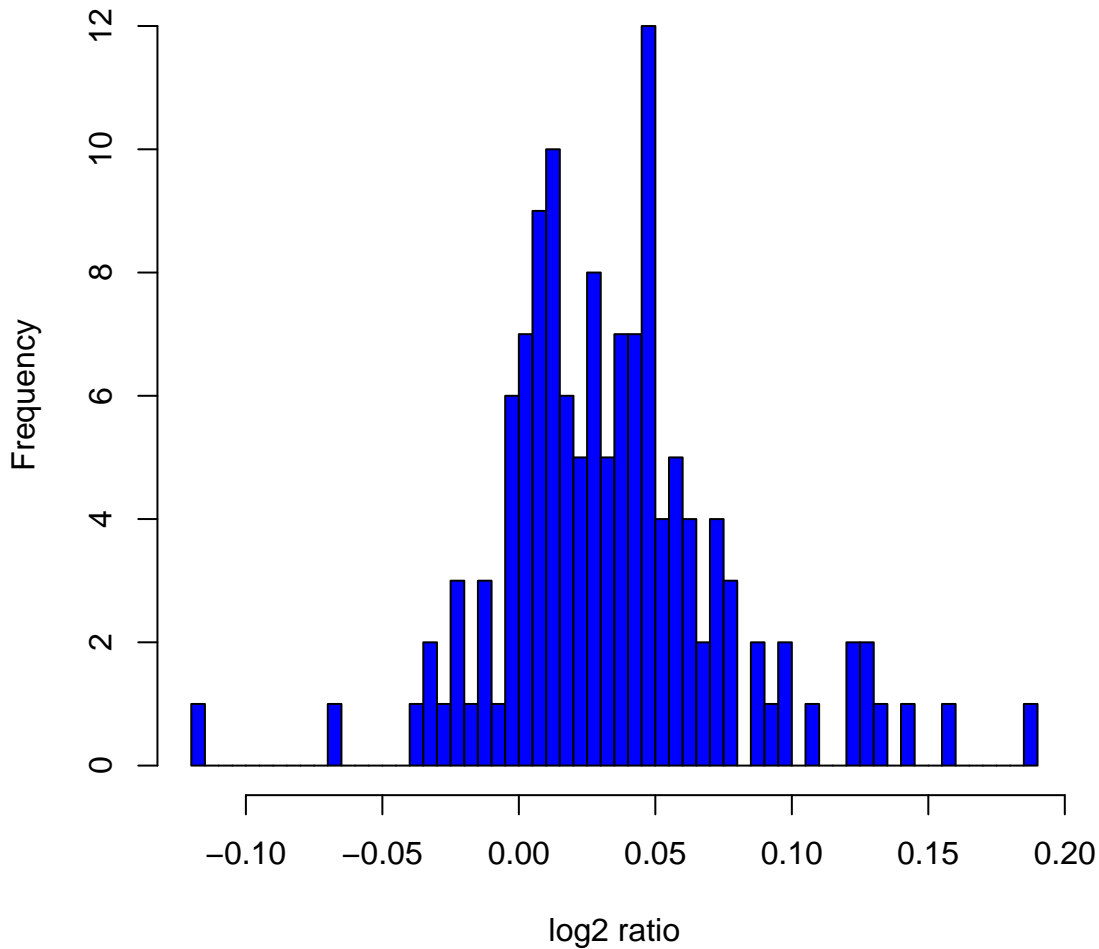
Histogram of \log_2 ratios in 142 HapMap male samples at clone ChrXtp-23C3
