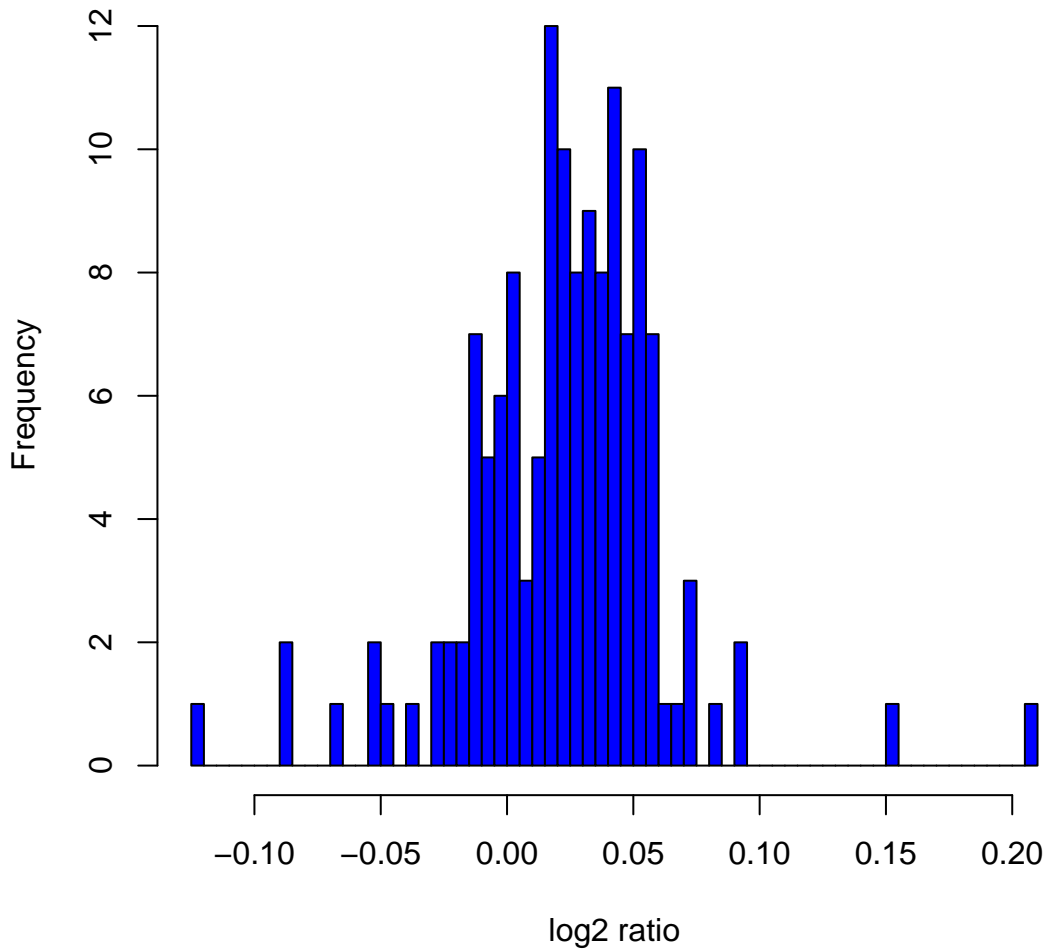
Histogram of log 2 ratios in 142 HapMap male samples at clone ChrXtp-23D9
