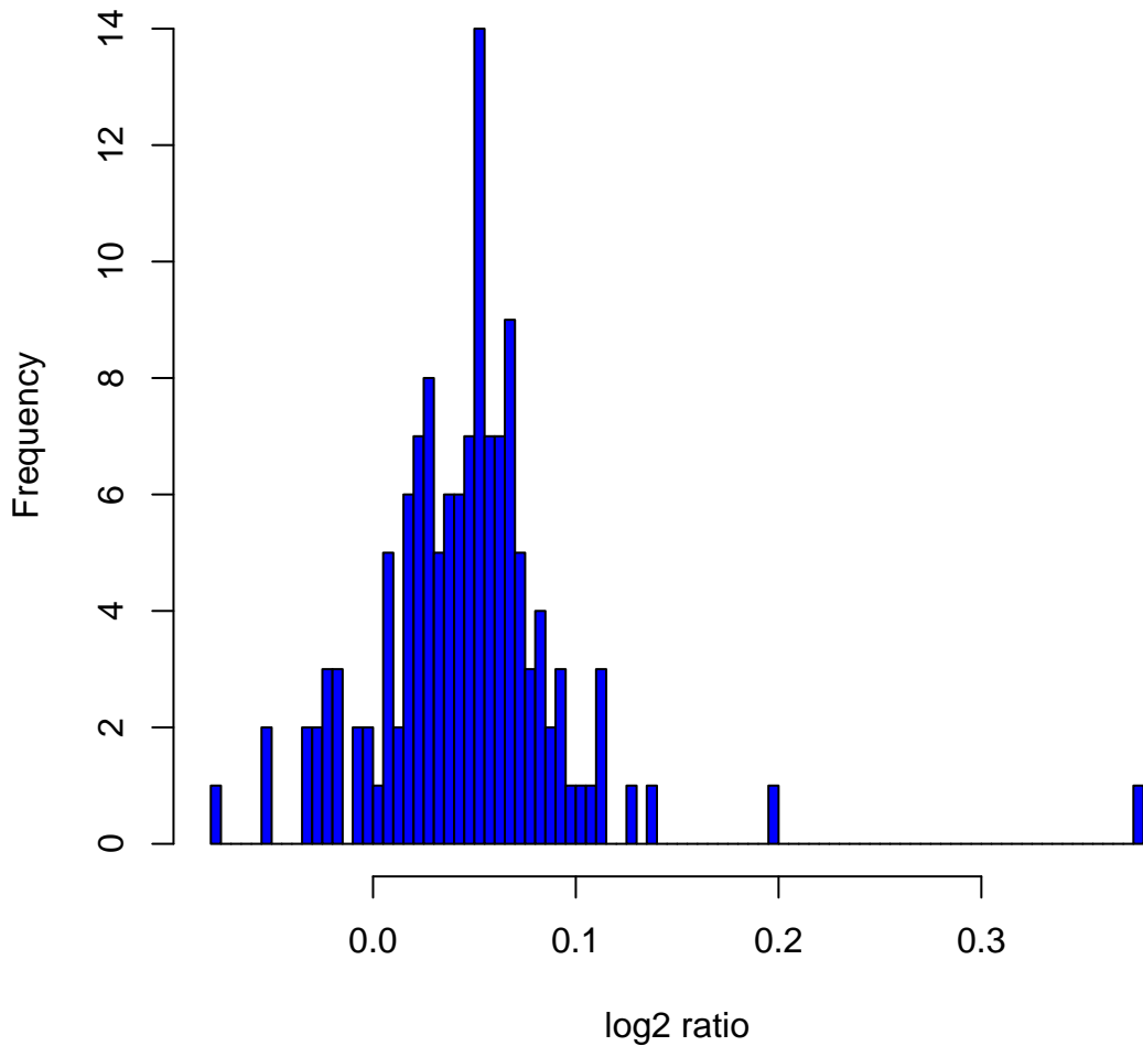
Histogram of \log_2 ratios in 142 HapMap male samples at clone ChrXtp-25B6
