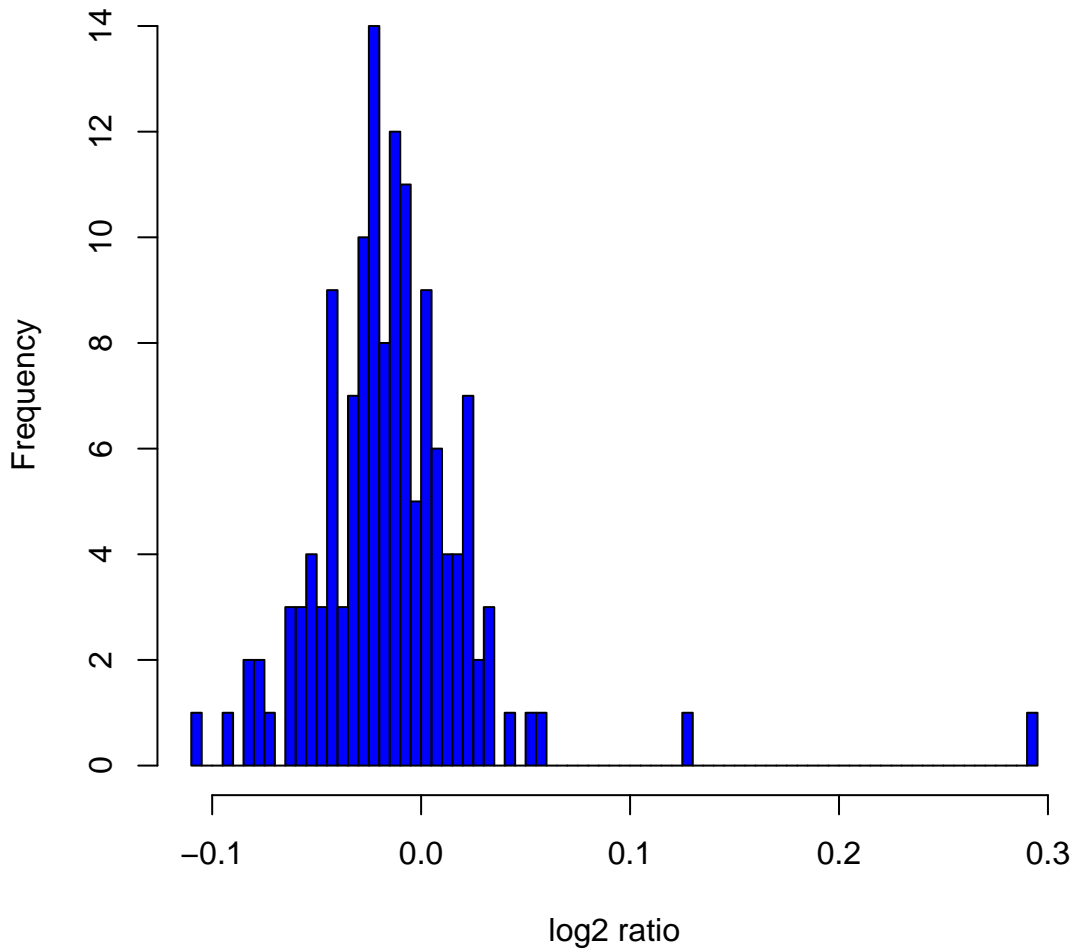
Histogram of \log_2 ratios in 142 HapMap male samples at clone ChrXtp-2B11
