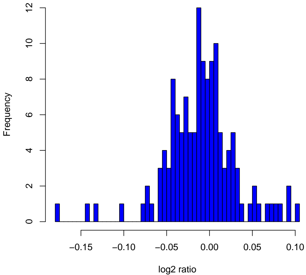
Histogram of log2ratios in 142 HapMap male samples at clone ChrXtp-2E5
